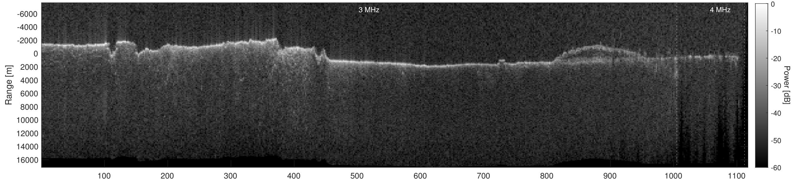
Orbit 12036, Depth-Corrected Cluttergram
