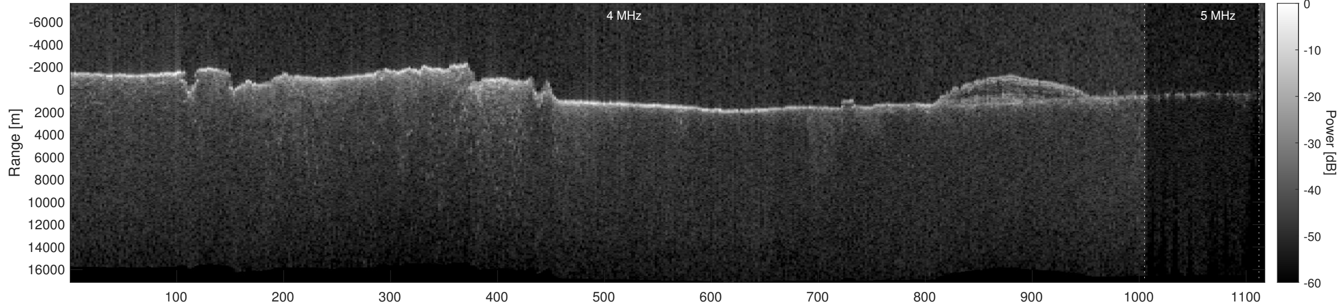
Orbit 12036, Optimized, Window, Depth-Corrected, Channel 2
