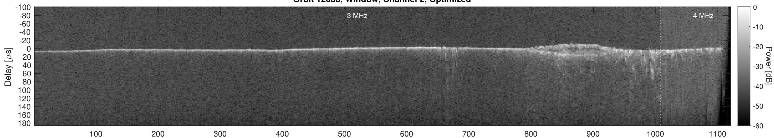
Orbit 12038, Cluttergram
