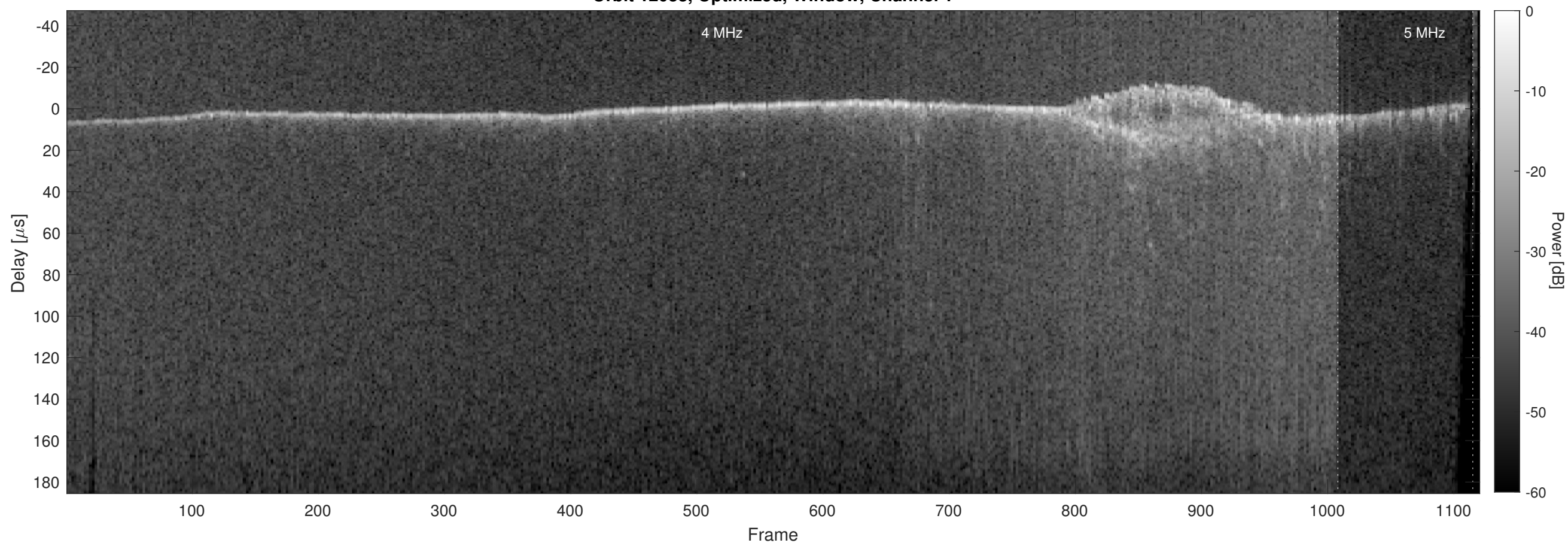
Orbit 12038, Optimized, Window, Channel 2
