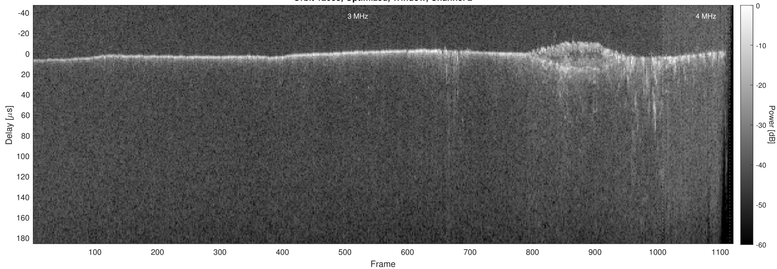
Orbit 12038, Optimized, Window, Channel 2
