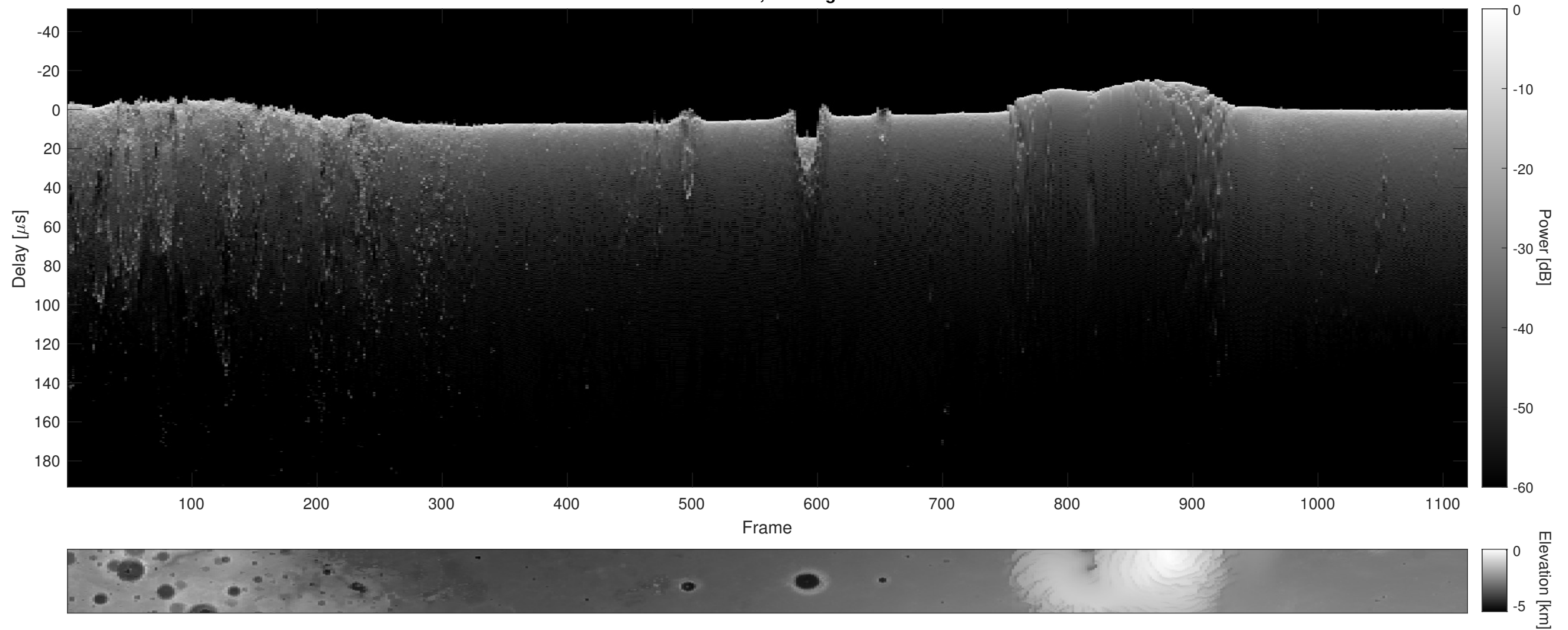
Orbit 12039, Cluttergram
