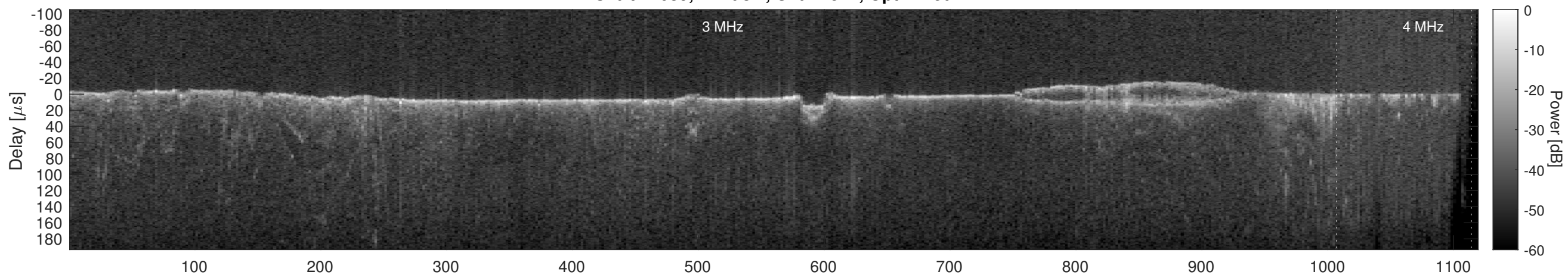
Orbit 12039, Cluttergram
