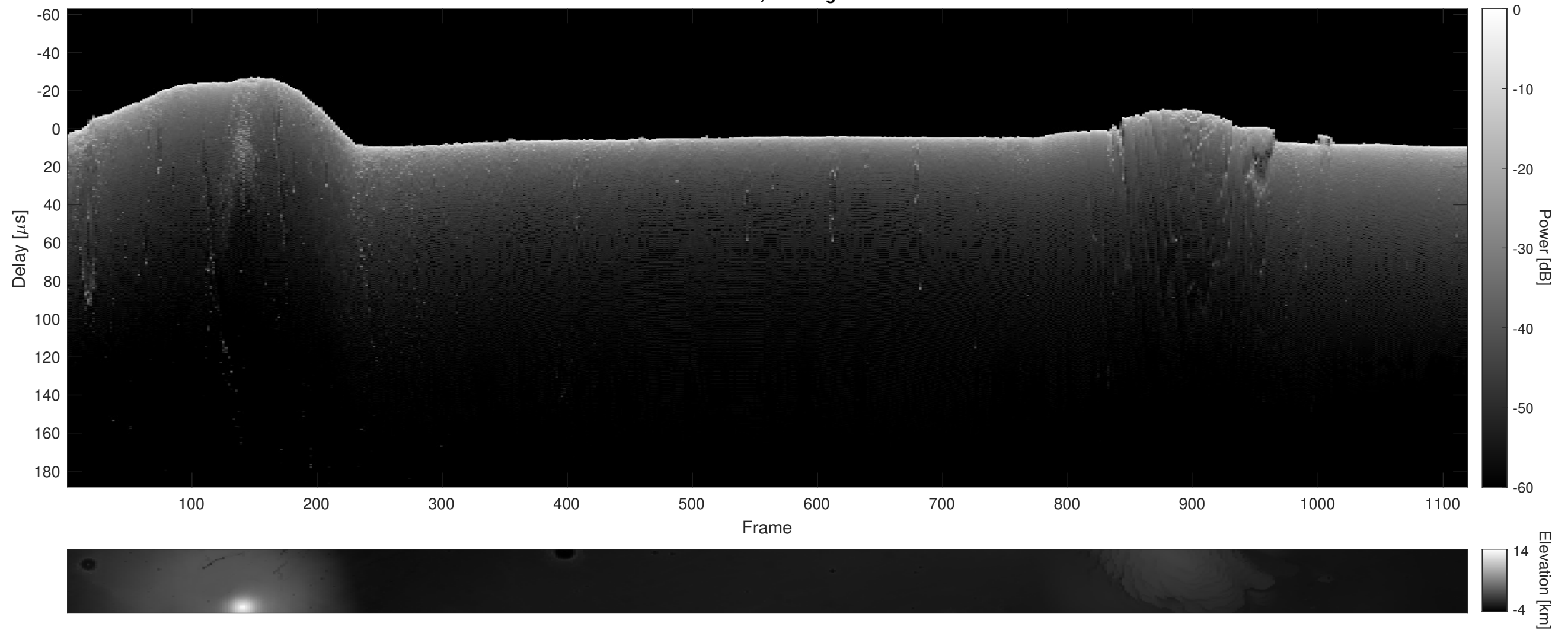
Orbit 12041, Cluttergram
