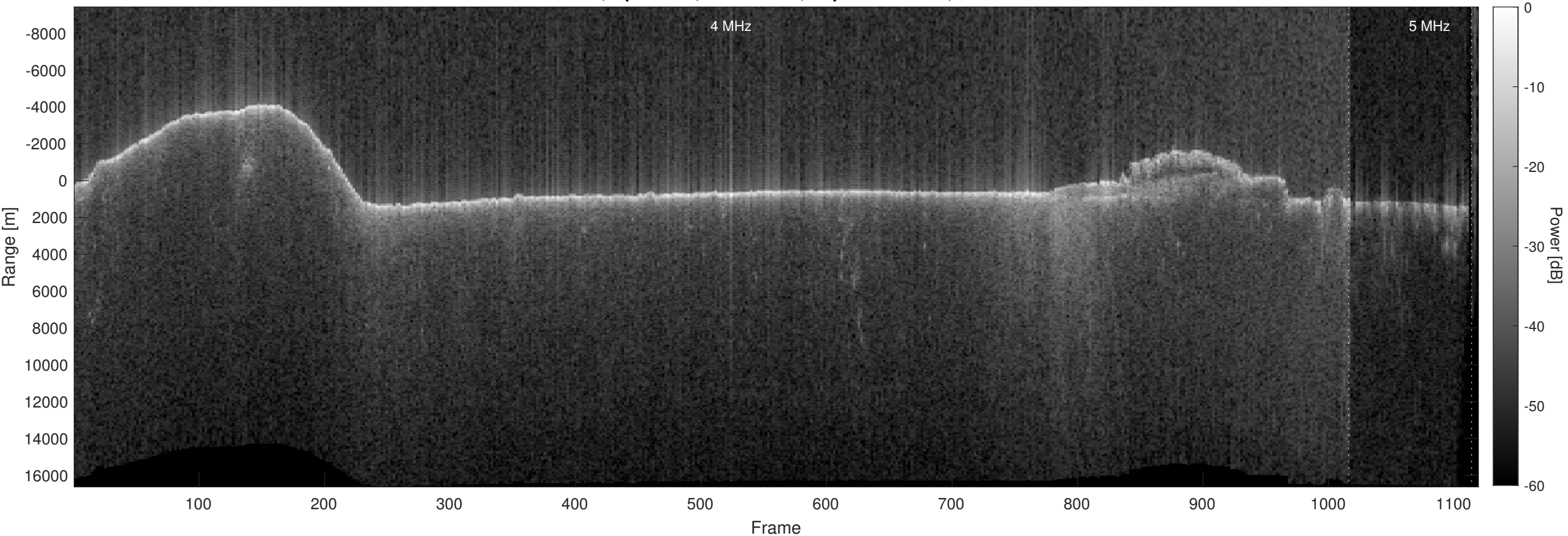
Orbit 12041, Optimized, No Window, Depth-Corrected, Channel 2
