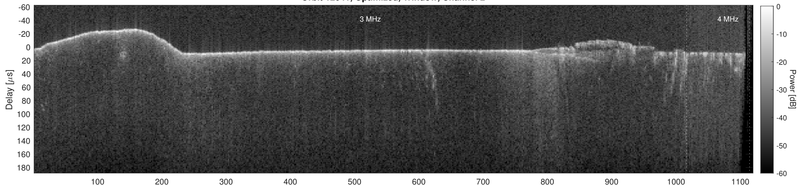
Orbit 12041, Cluttergram
