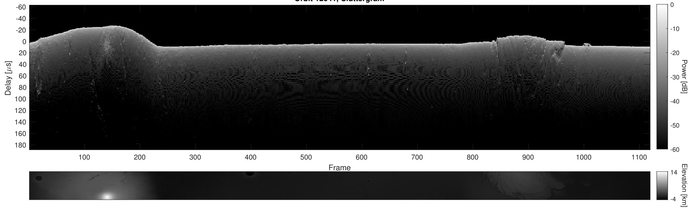
Orbit 12041, Cluttergram
