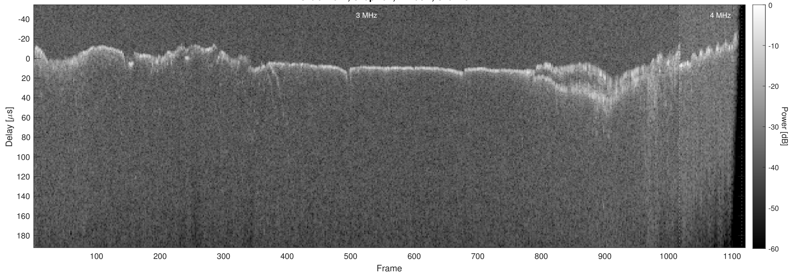
Orbit 12042, Chapman, Window, Channel 2
