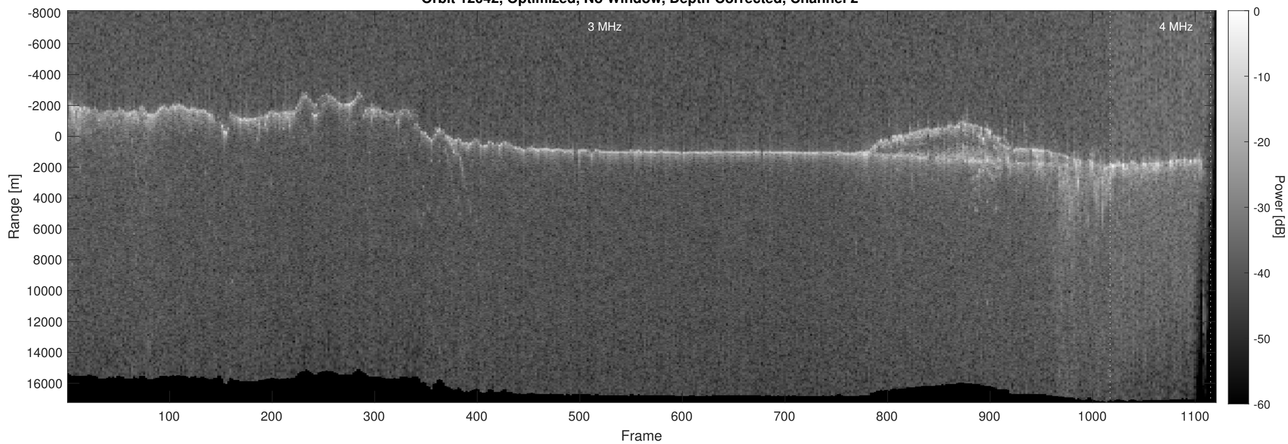
Orbit 12042, Optimized, No Window, Depth-Corrected, Channel 2
