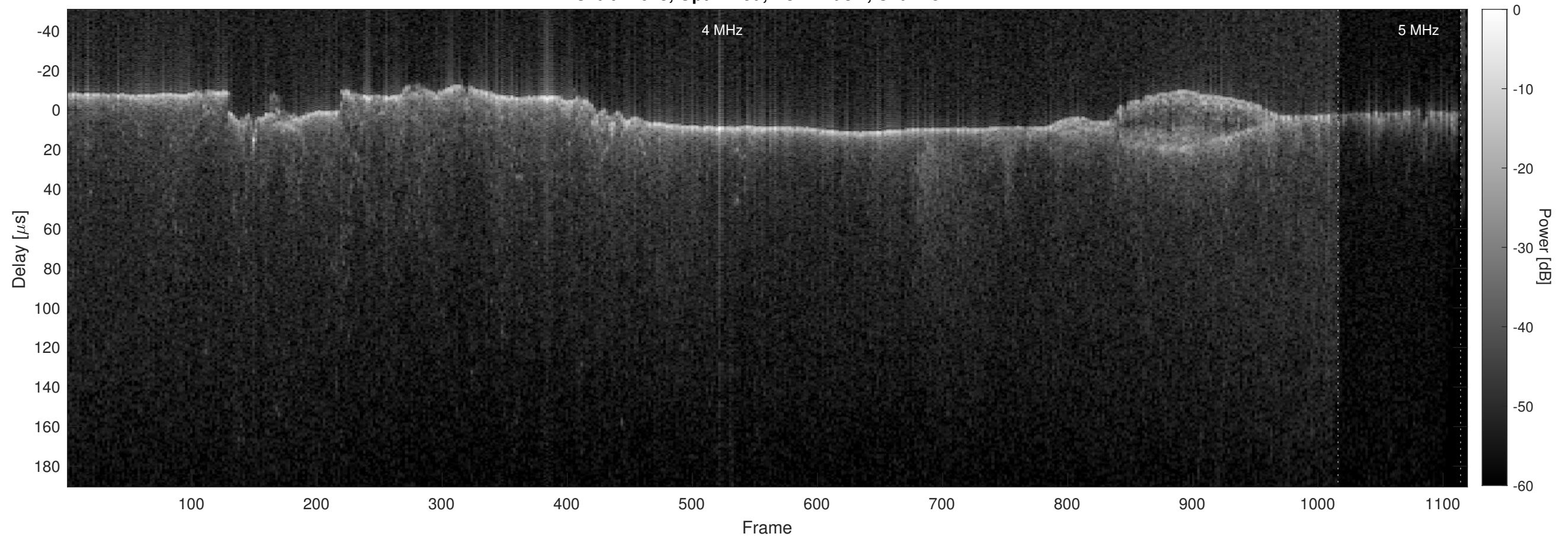
Orbit 12043, Optimized, No Window, Channel 2
