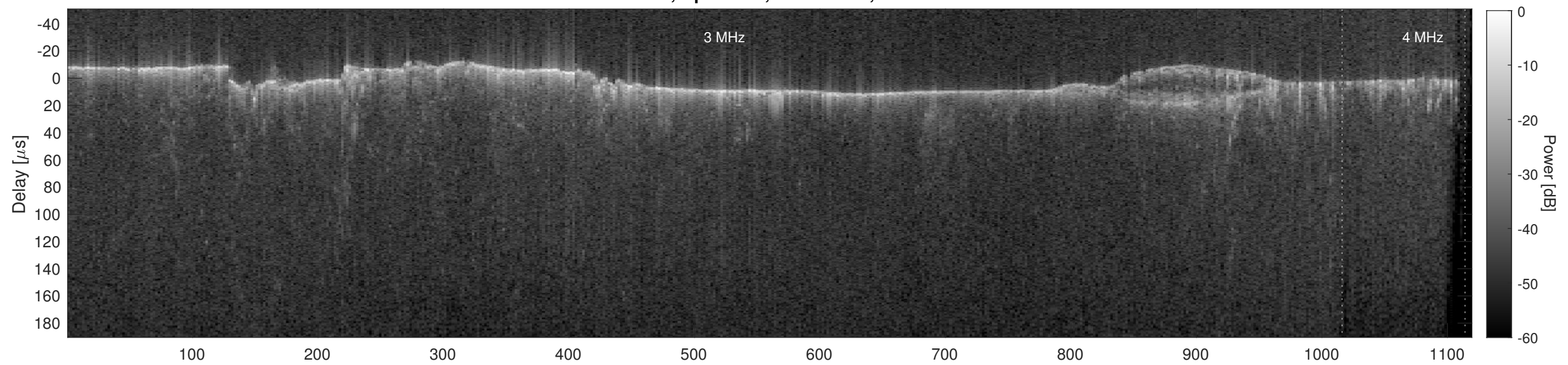
Orbit 12043, Cluttergram
