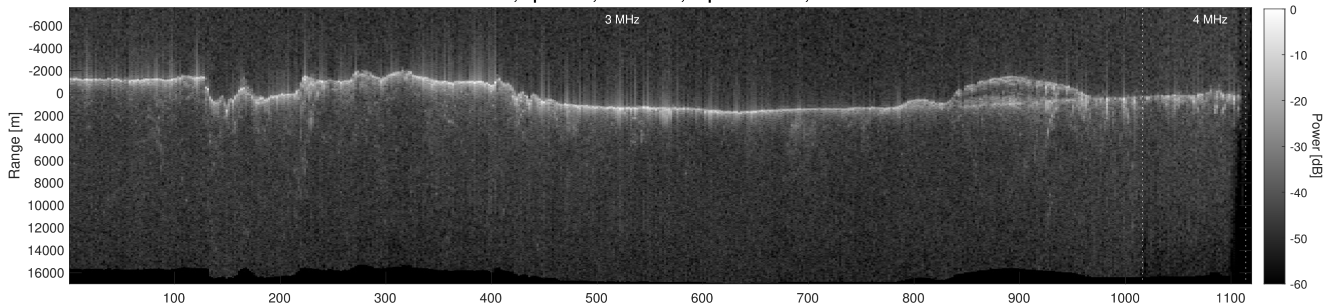
Orbit 12043, Depth-Corrected Cluttergram
