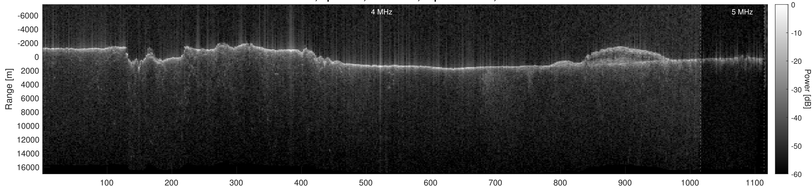
Orbit 12043, Optimized, No Window, Depth-Corrected, Channel 2
