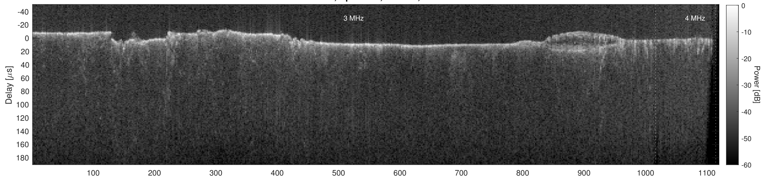
Orbit 12043, Cluttergram
