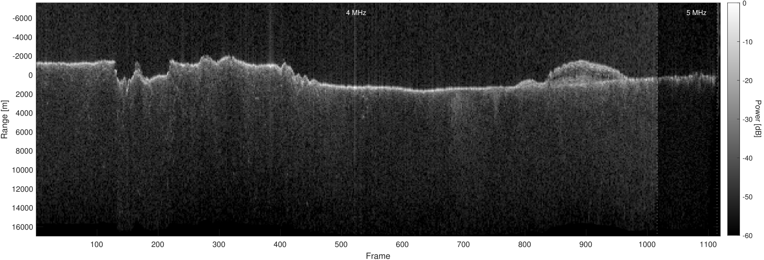
Orbit 12043, Optimized, Window, Depth-Corrected, Channel 2
