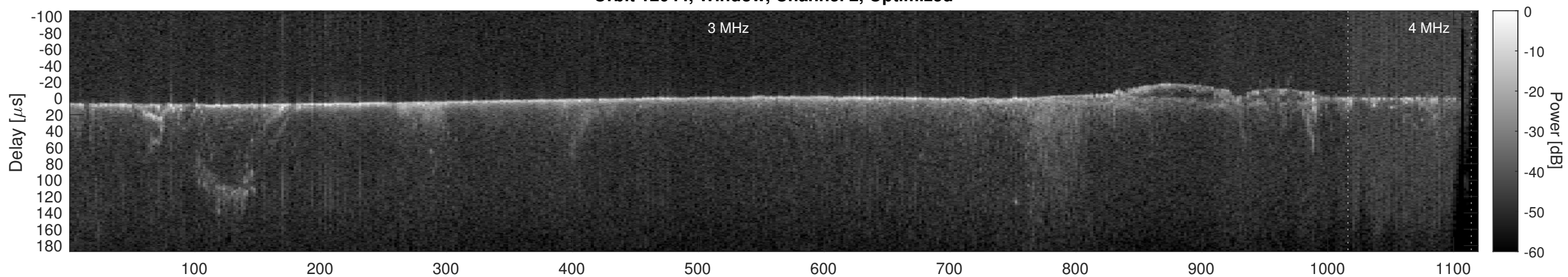
Orbit 12044, Cluttergram
