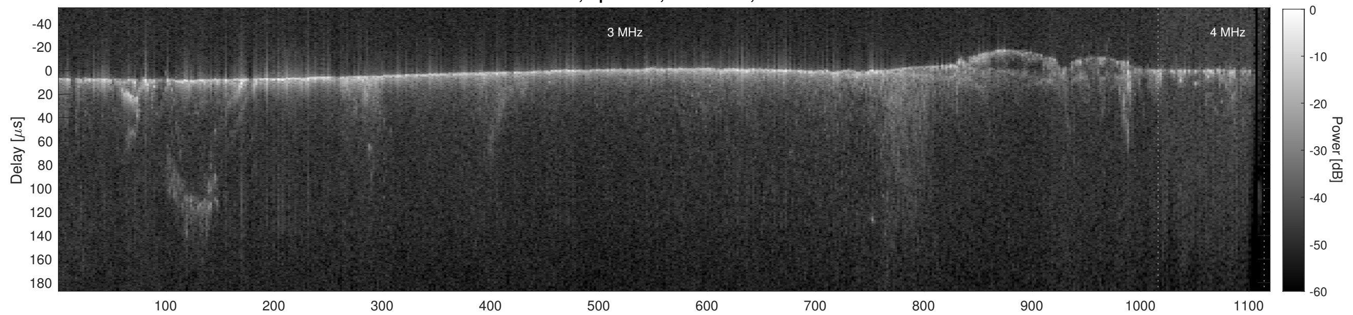
Orbit 12044, Cluttergram
