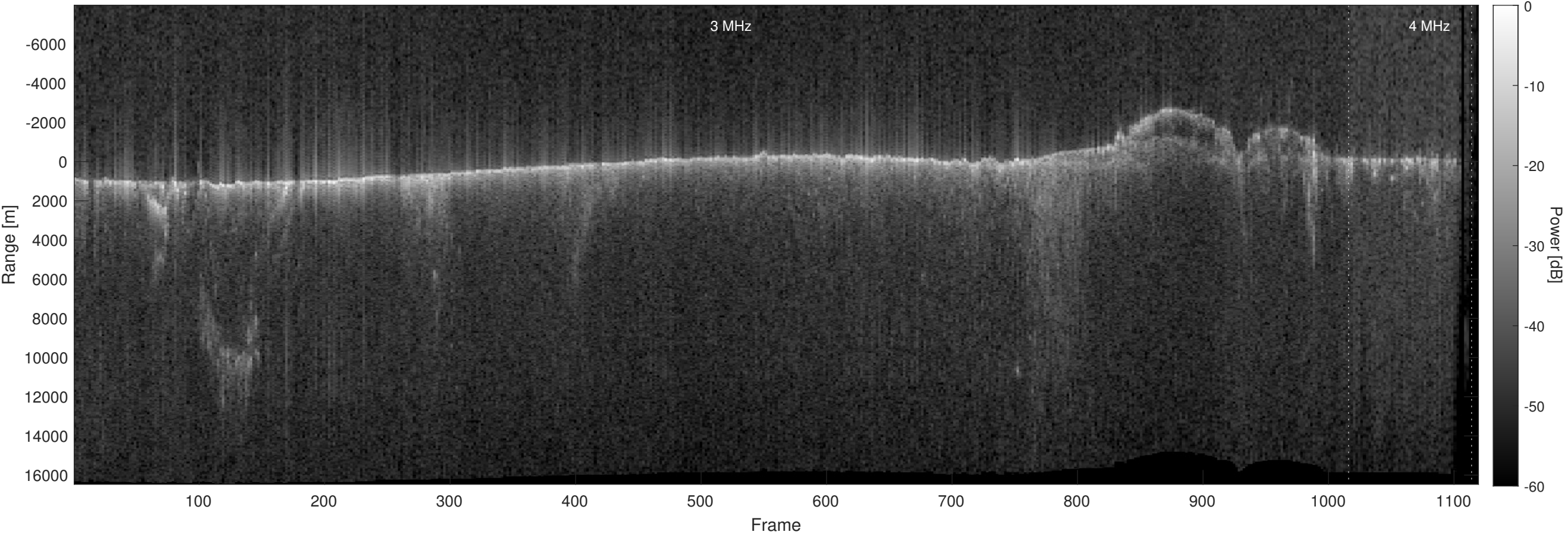
Orbit 12044, Optimized, No Window, Depth-Corrected, Channel 2
