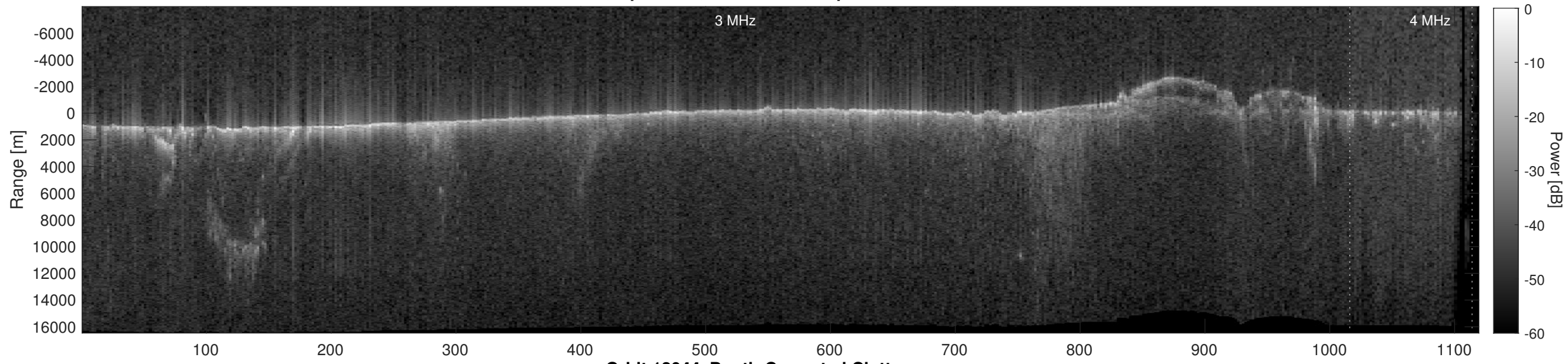
Orbit 12044, Depth-Corrected Cluttergram
