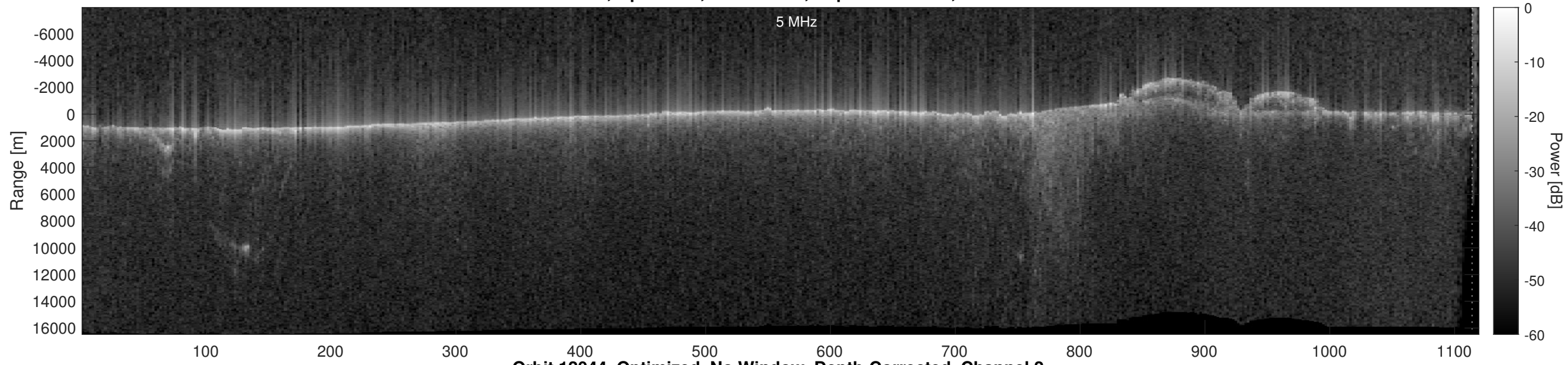
Orbit 12044, Optimized, No Window, Depth-Corrected, Channel 2
