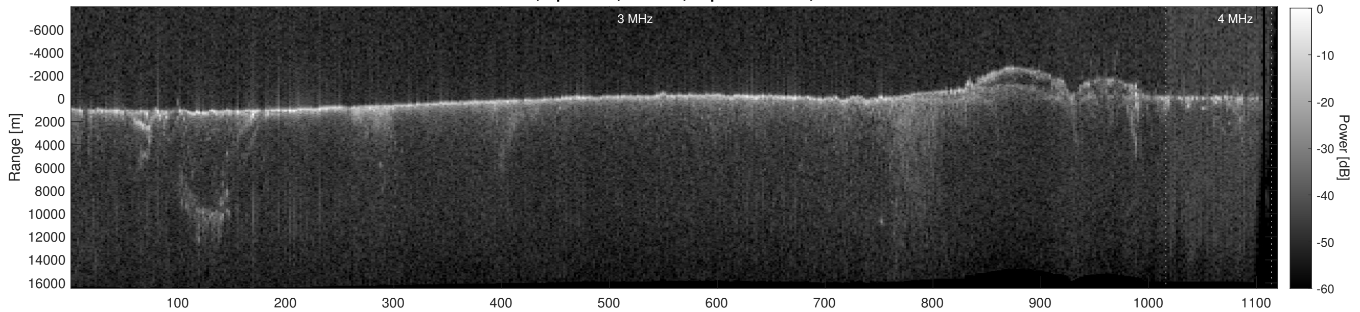
Orbit 12044, Depth-Corrected Cluttergram
