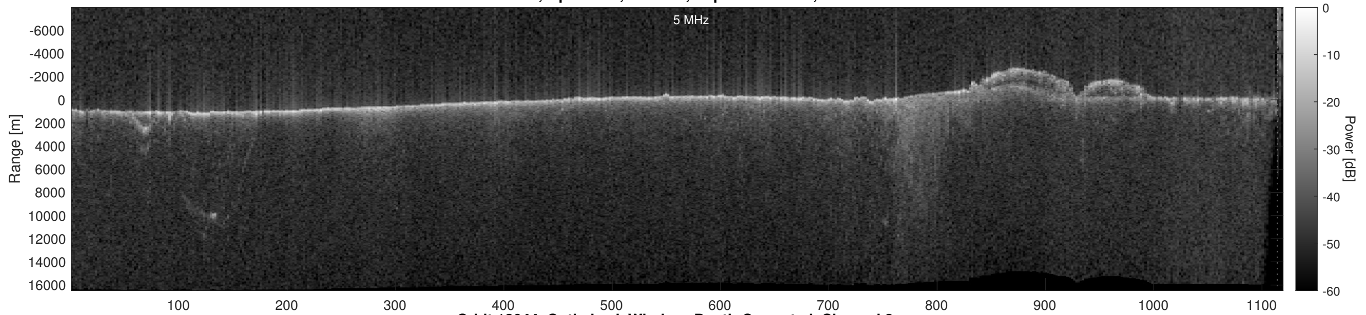
Orbit 12044, Optimized, Window, Depth-Corrected, Channel 2
