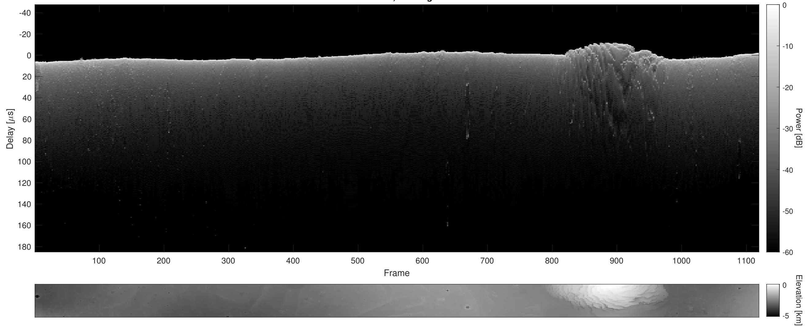
Orbit 12045, Cluttergram
