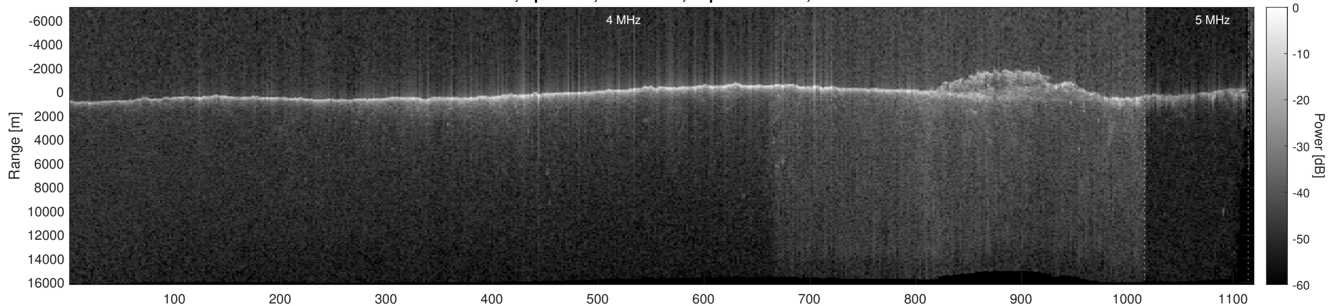
Orbit 12045, Optimized, No Window, Depth-Corrected, Channel 2
