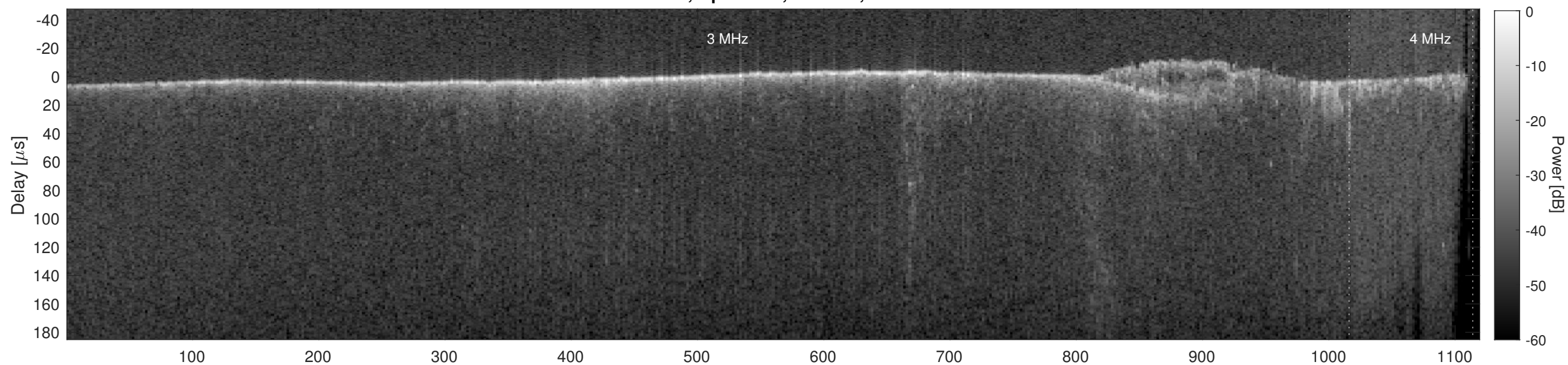
Orbit 12045, Cluttergram
