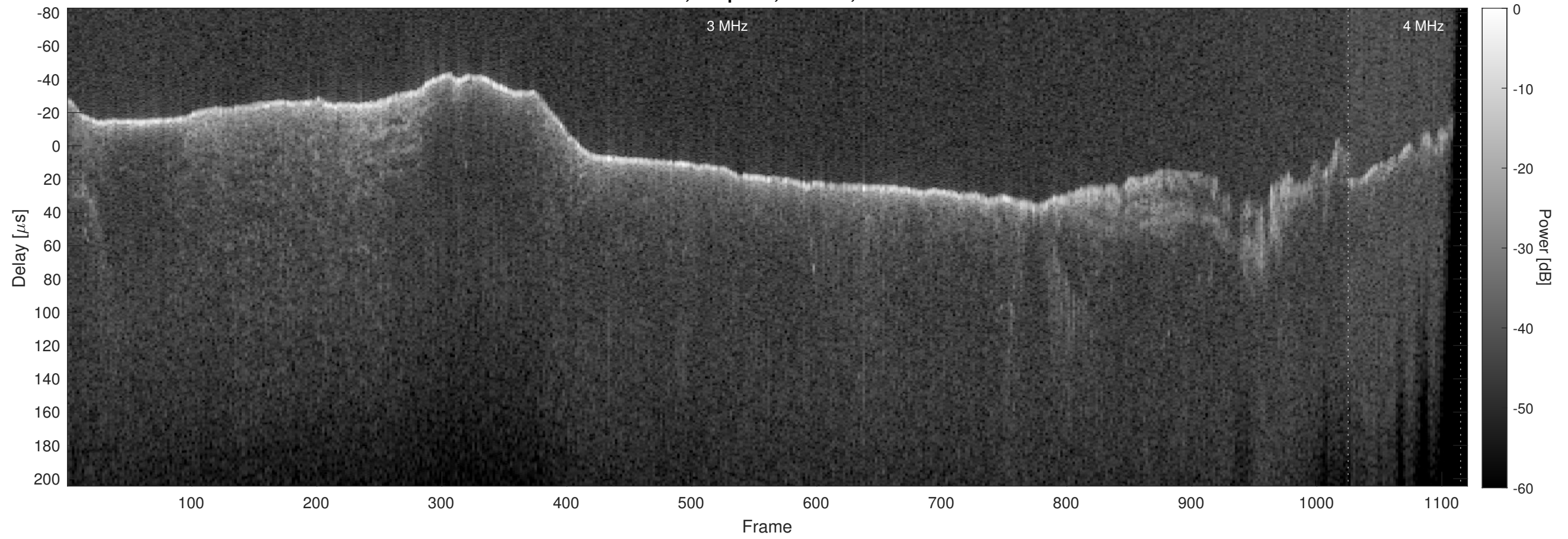
Orbit 12047, Chapman, Window, Channel 2
