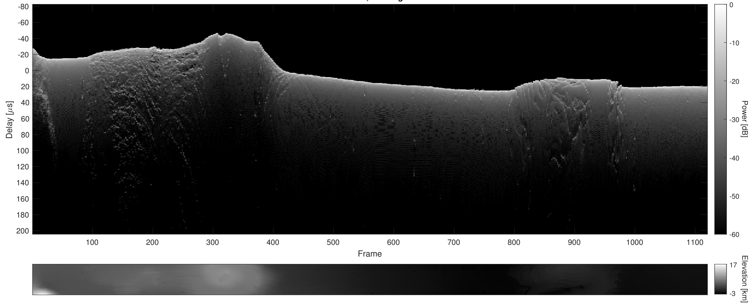
Orbit 12047, Cluttergram
