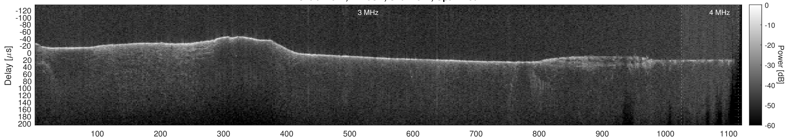
Orbit 12047, Cluttergram
