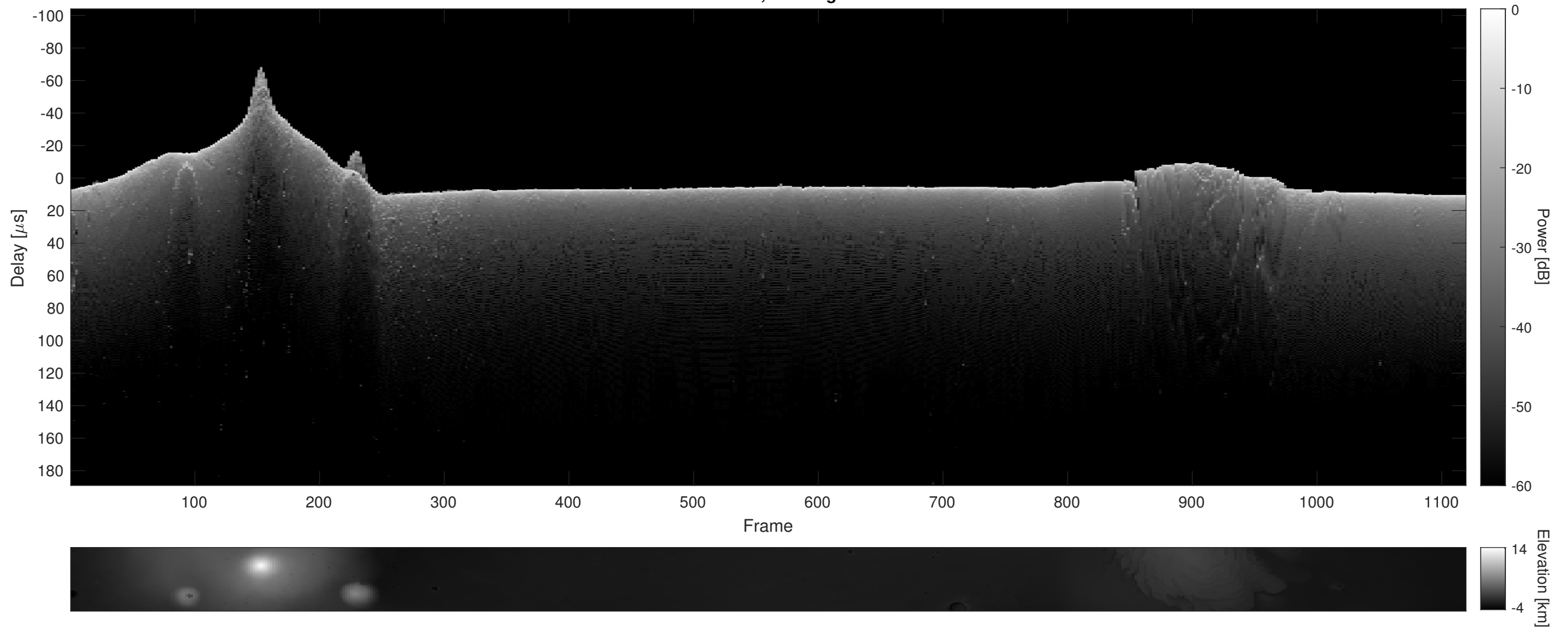
Orbit 12048, Cluttergram
