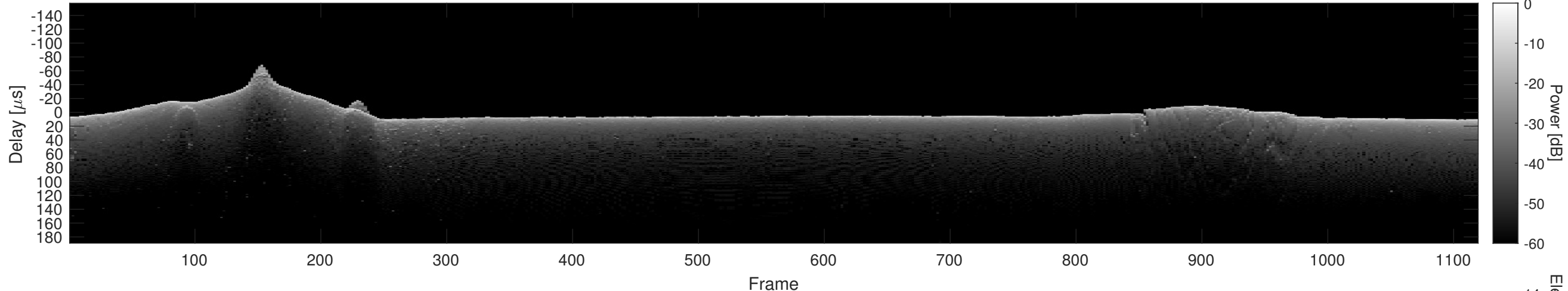
Orbit 12048, Cluttergram
