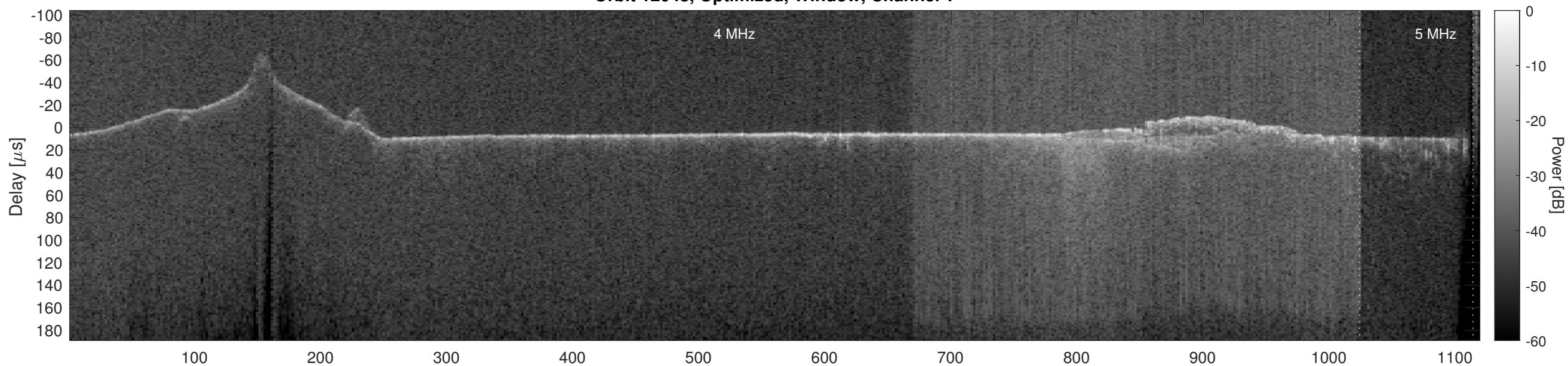
Orbit 12048, Optimized, Window, Channel 2
