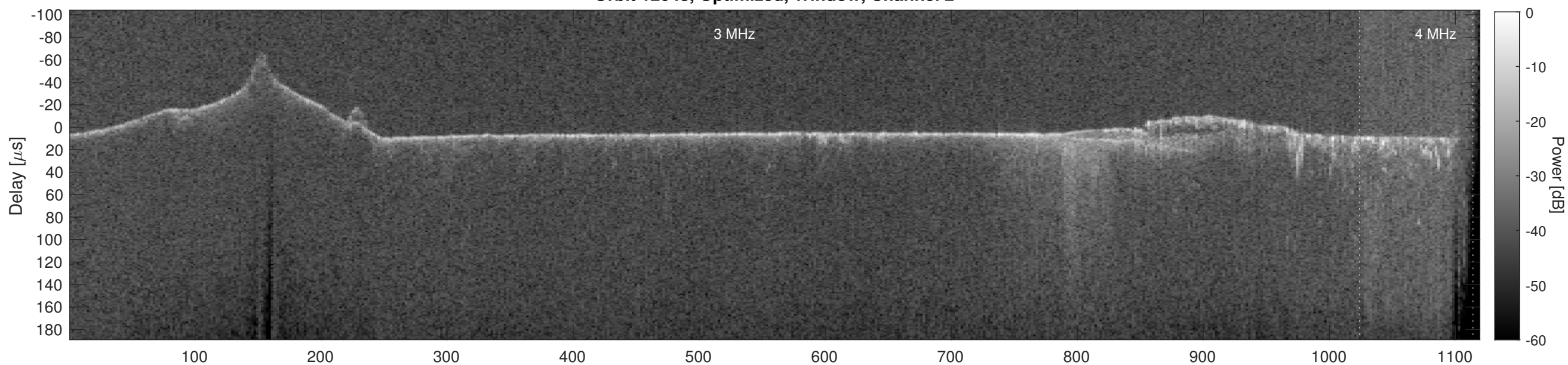
Orbit 12048, Cluttergram
