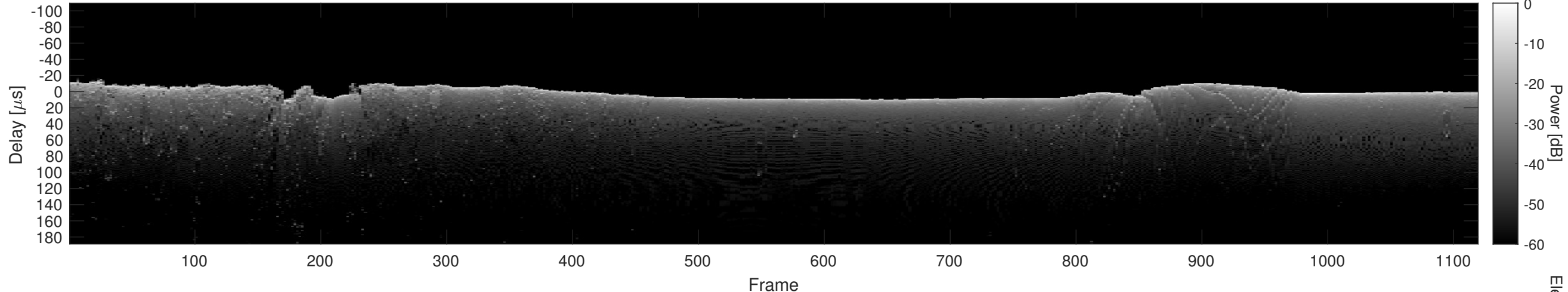
Orbit 12050, Cluttergram
