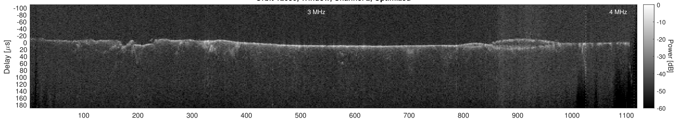
Orbit 12050, Cluttergram
