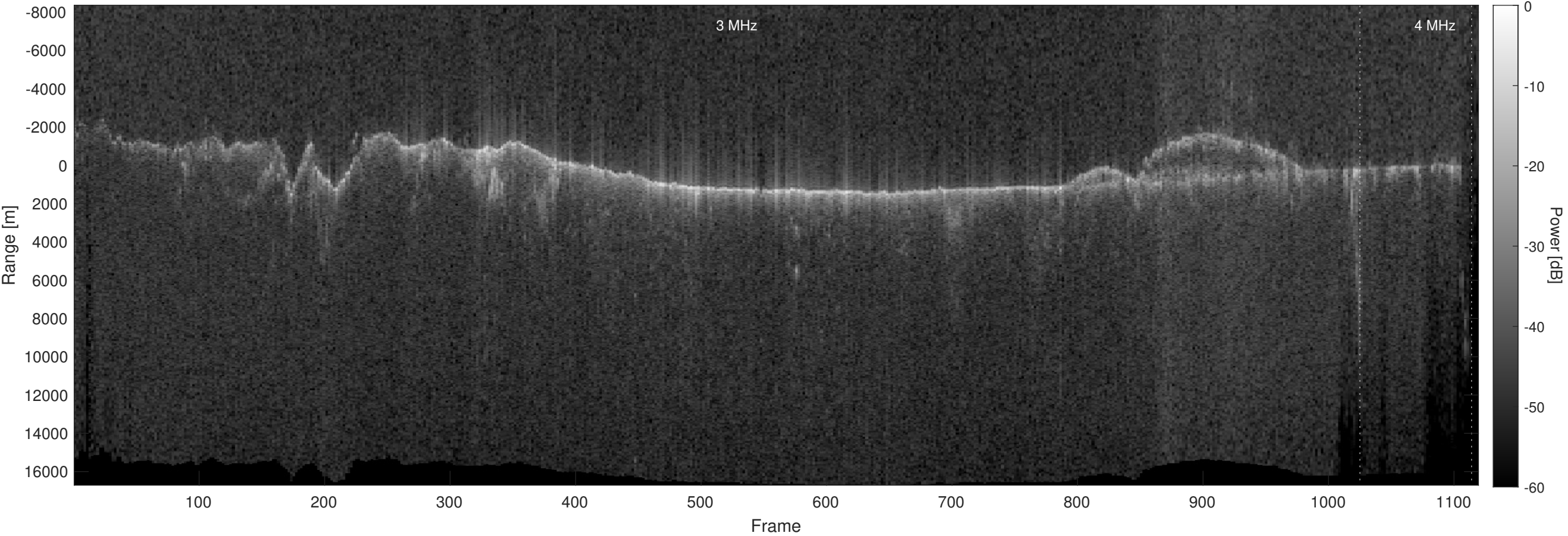
Orbit 12050, Optimized, No Window, Depth-Corrected, Channel 2
