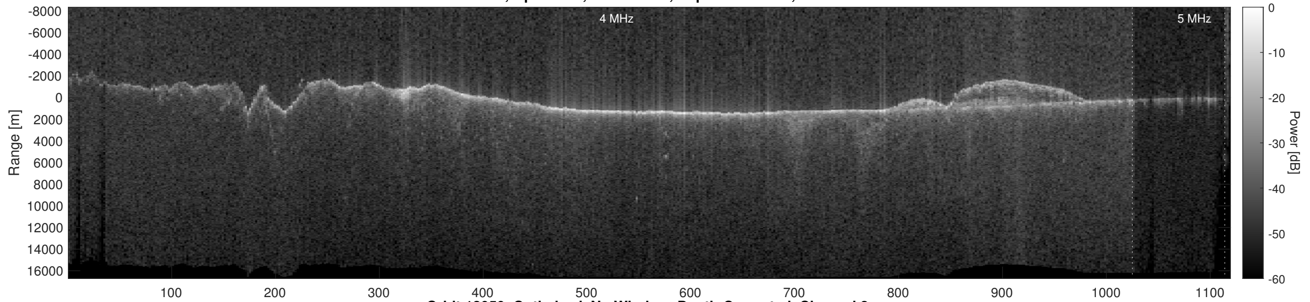
Orbit 12050, Optimized, No Window, Depth-Corrected, Channel 2
