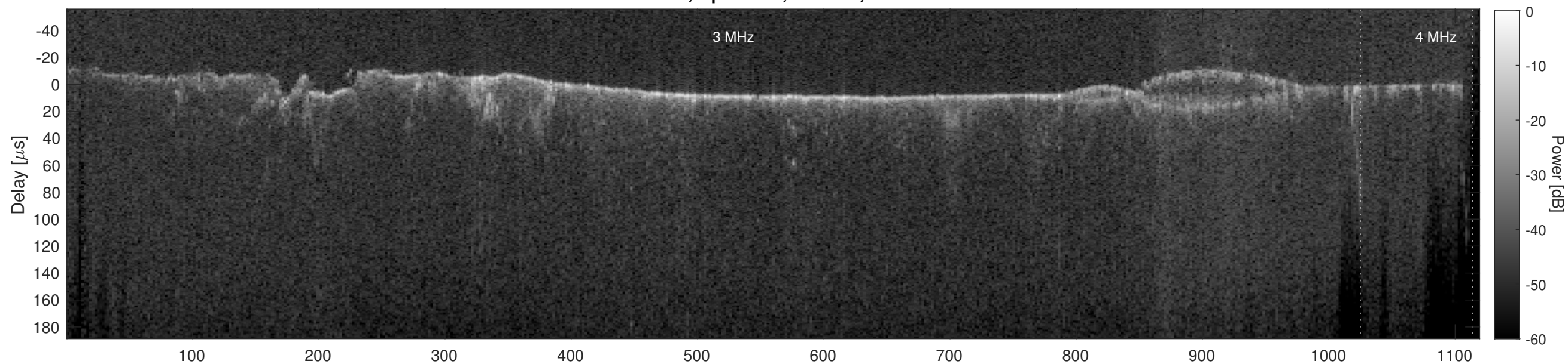
Orbit 12050, Cluttergram
