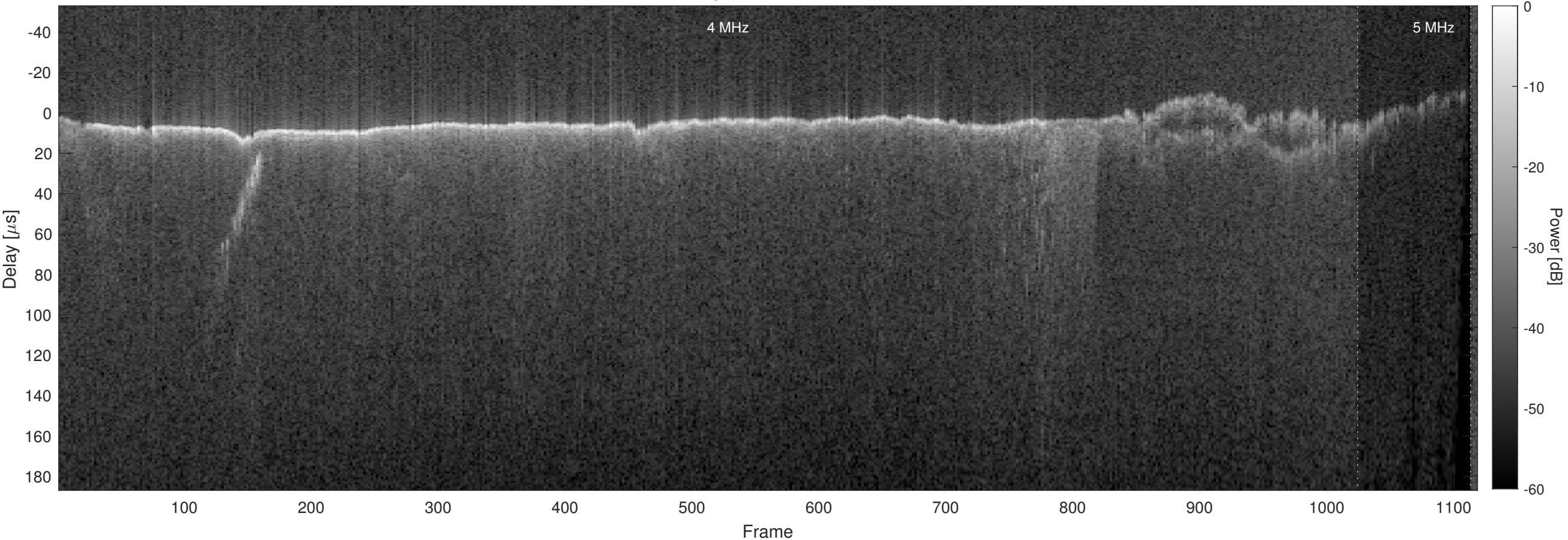
Orbit 12051, Chapman, No Window, Channel 2
