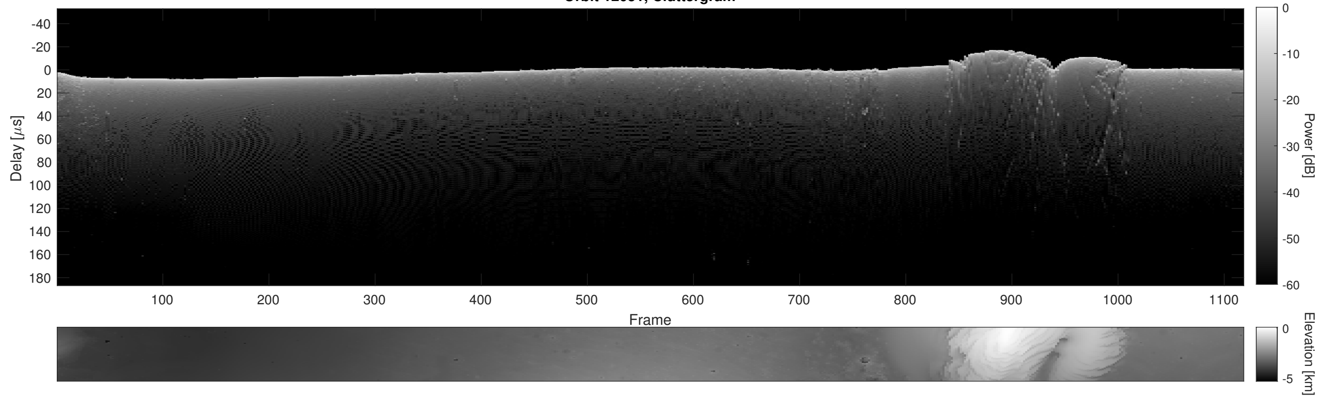
Orbit 12051, Cluttergram
