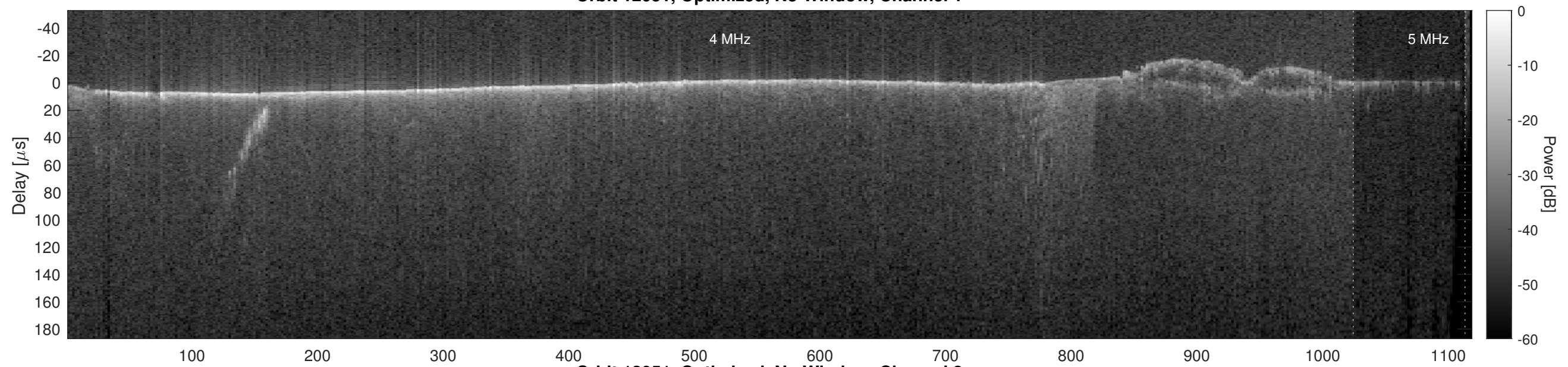
Orbit 12051, Optimized, No Window, Channel 2
