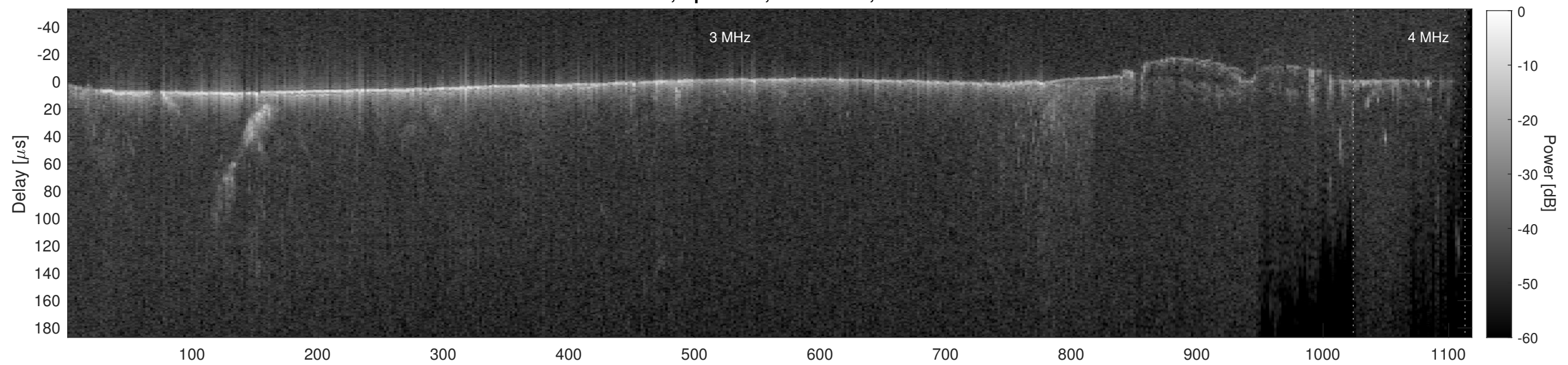
Orbit 12051, Cluttergram
