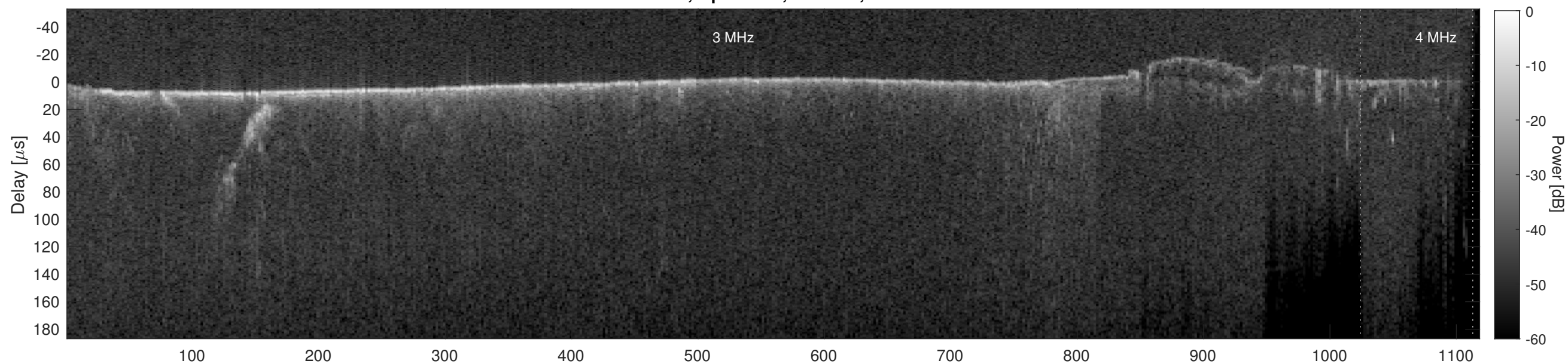
Orbit 12051, Cluttergram
