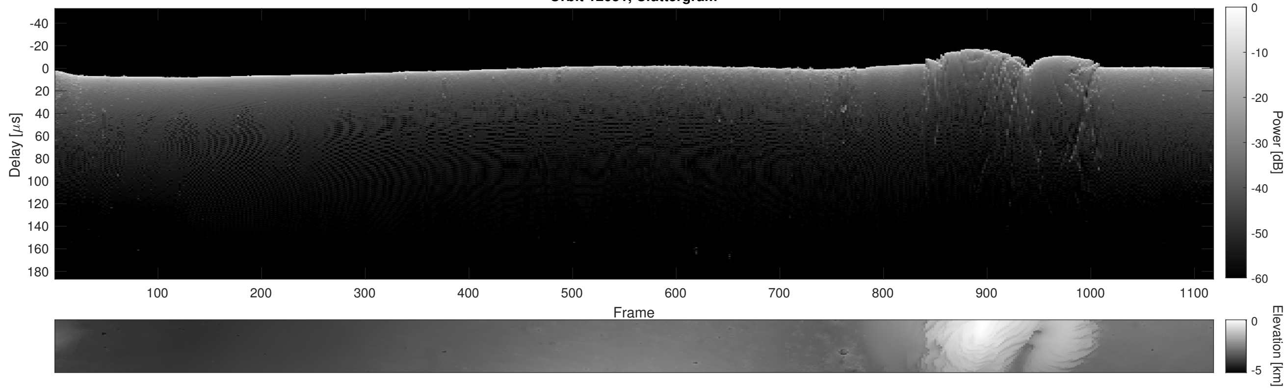
Orbit 12051, Cluttergram
