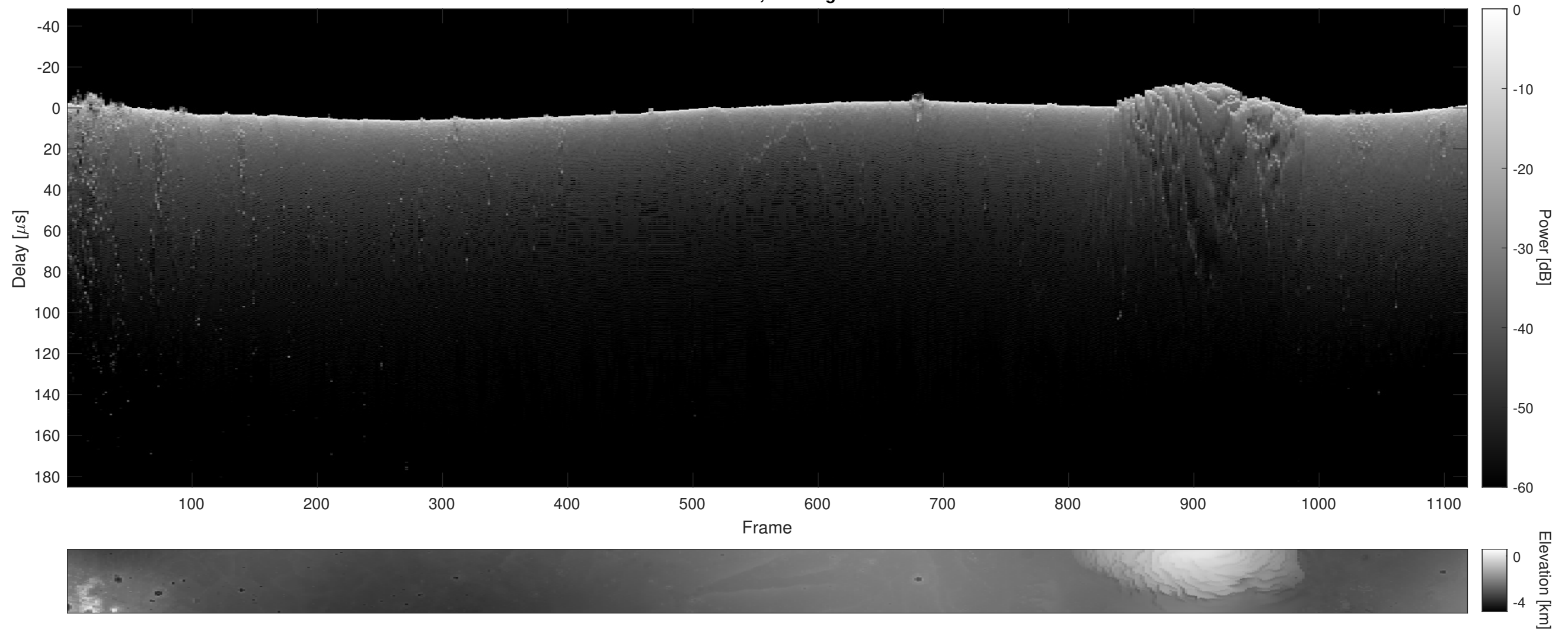
Orbit 12052, Cluttergram
