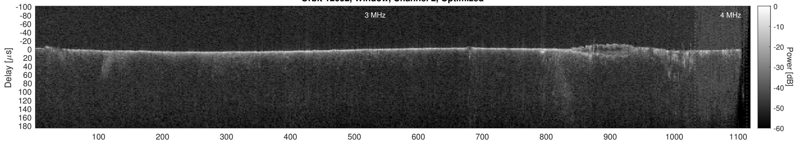
Orbit 12052, Cluttergram
