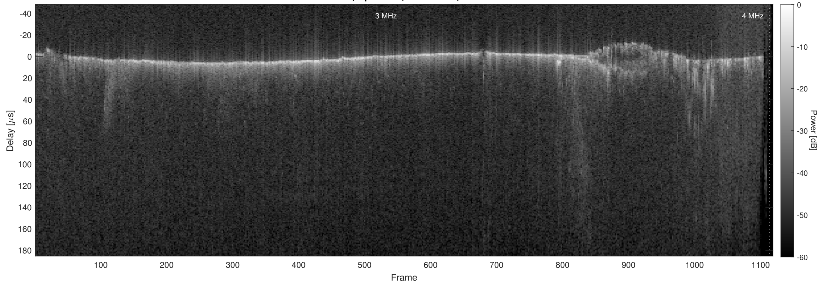
Orbit 12052, Optimized, No Window, Channel 2
