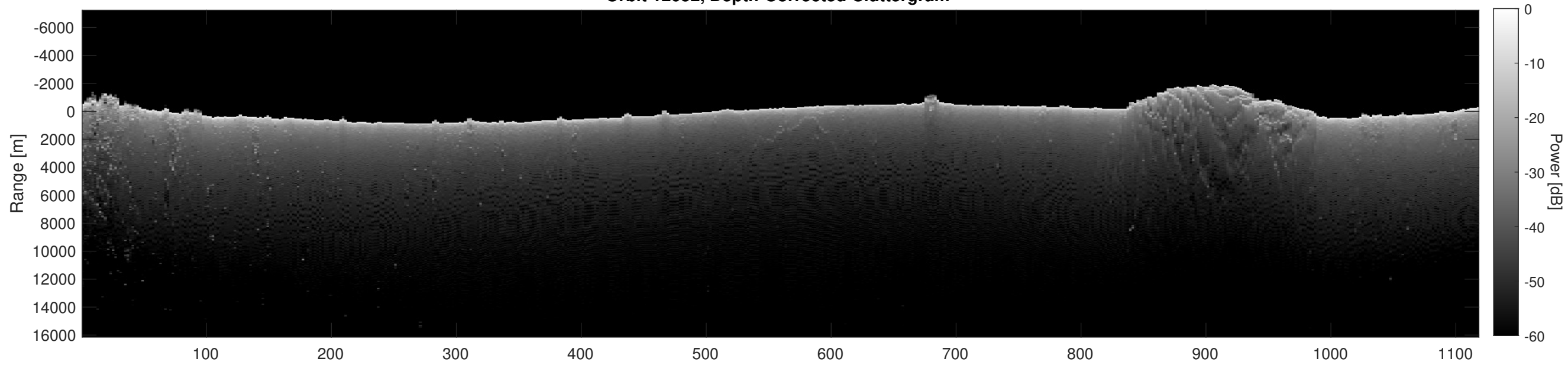
Orbit 12052, Depth-Corrected Cluttergram
