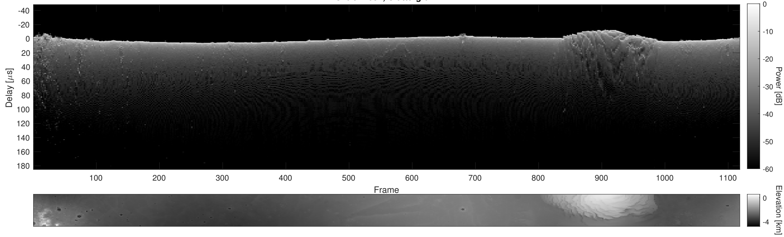
Orbit 12052, Cluttergram
