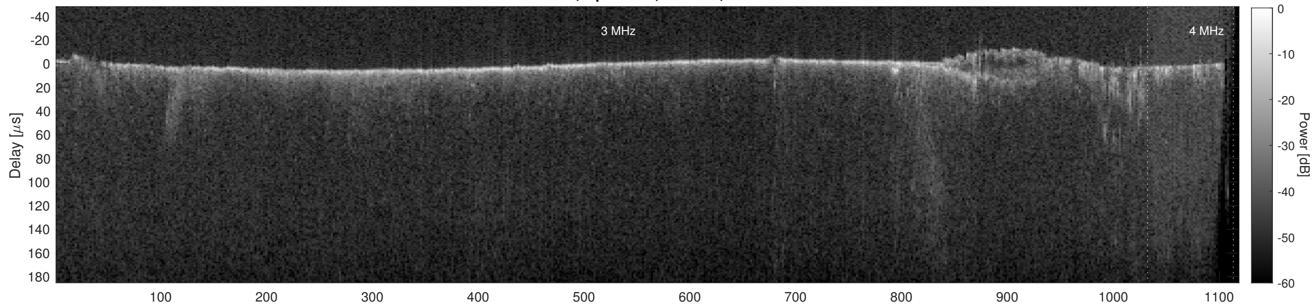
Orbit 12052, Cluttergram
