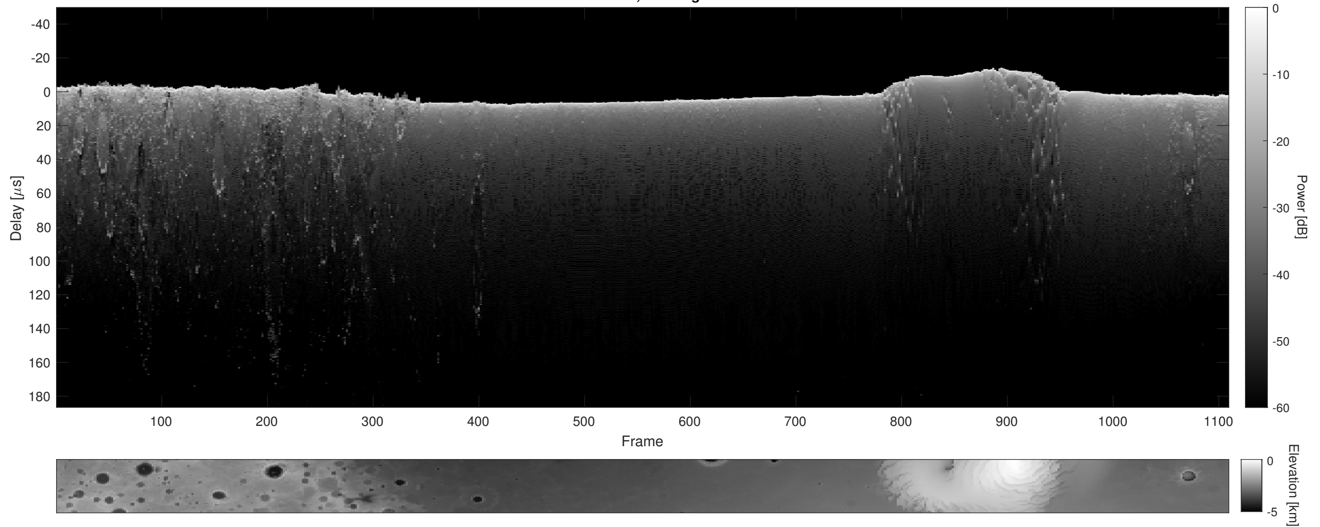
Orbit 12053, Cluttergram
