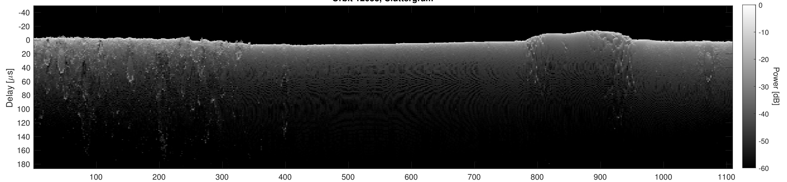
Orbit 12053, Cluttergram
