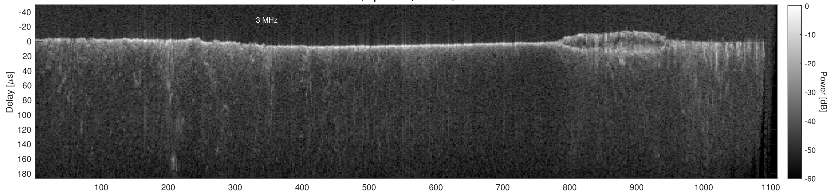
Orbit 12053, Cluttergram
