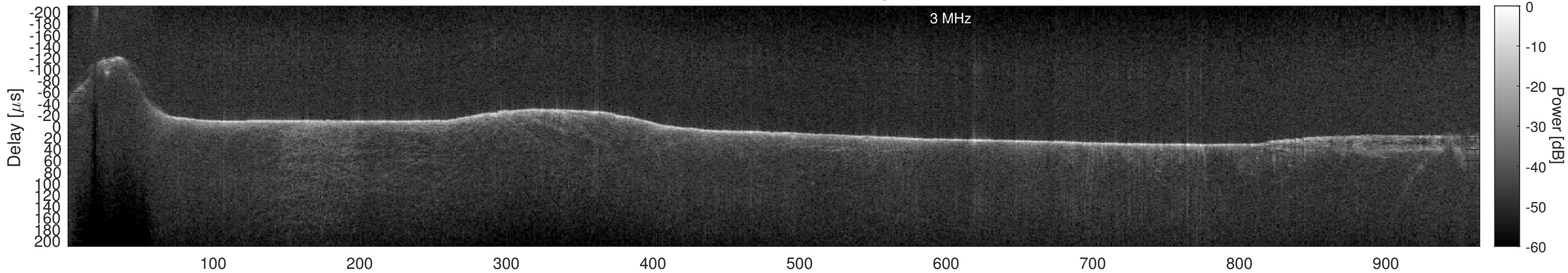
Orbit 12054, Cluttergram
