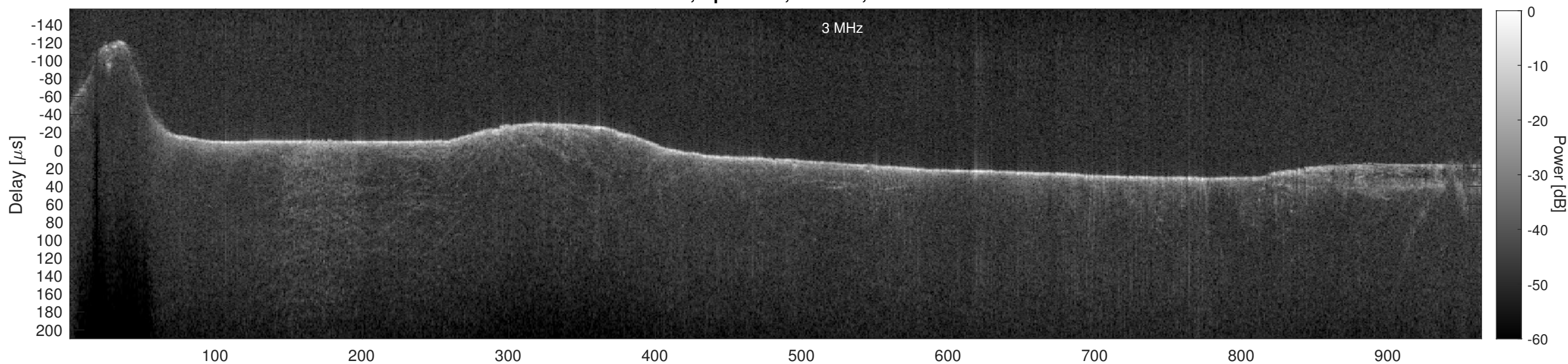
Orbit 12054, Cluttergram
