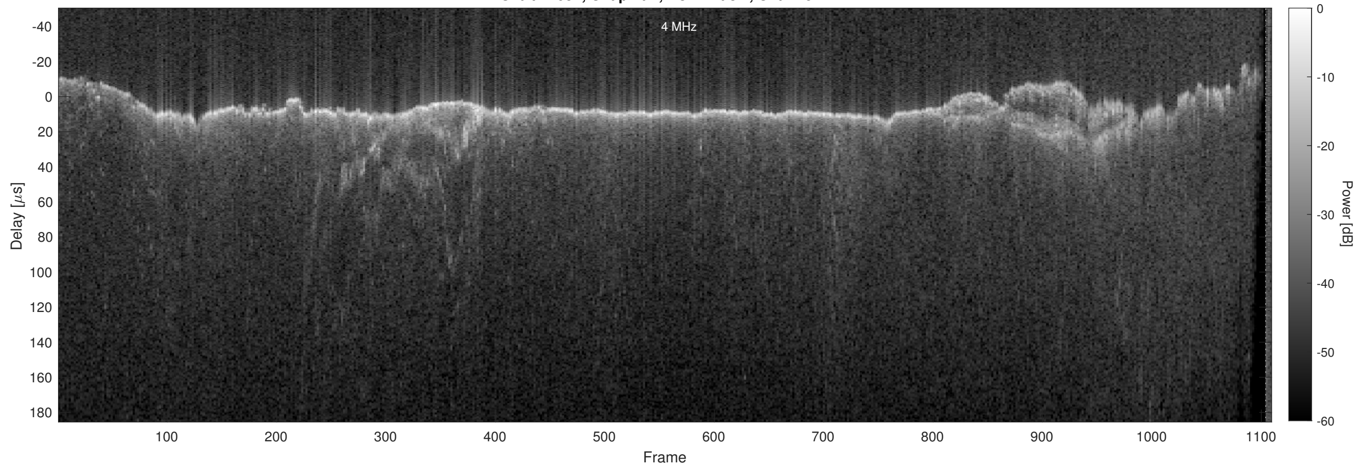
Orbit 12057, Chapman, No Window, Channel 2
