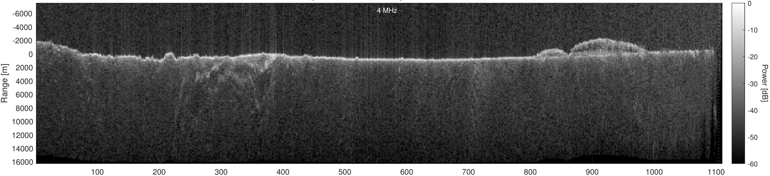
Orbit 12057, Optimized, Window, Depth-Corrected, Channel 2
