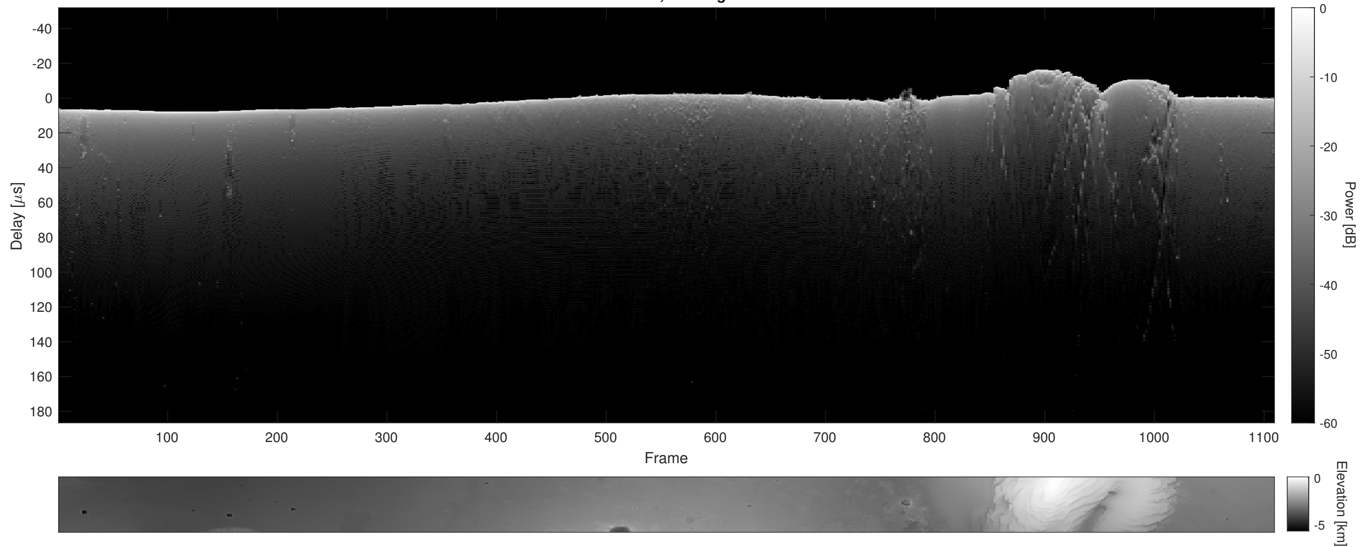
Orbit 12058, Cluttergram
